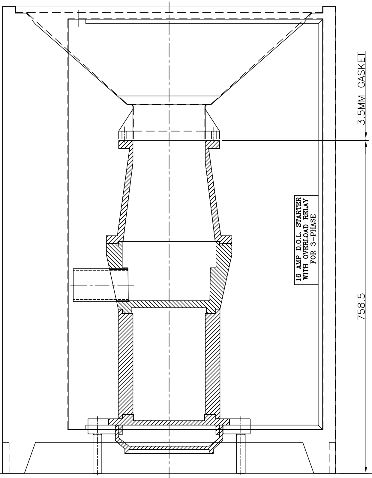
CRUSHAAL 3000 & 6000 FLOOR MOUNTED WITH STAND & S.S. CABINET
